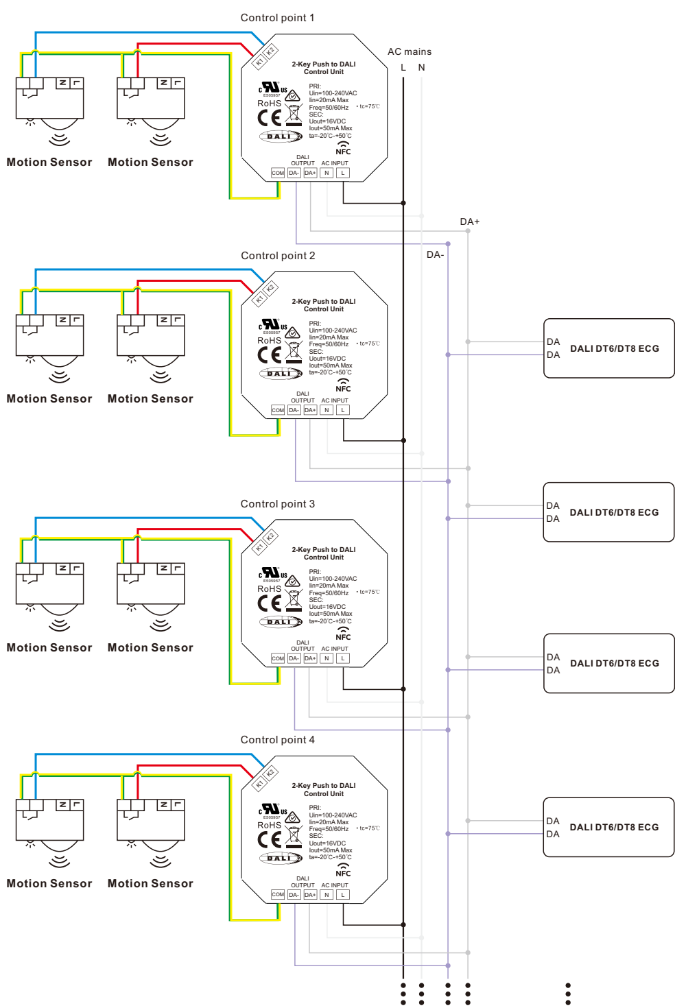
Figure 4: Wiring scheme to control up to 100 DALI ECGs (all 4 control units powered by AC mains)
