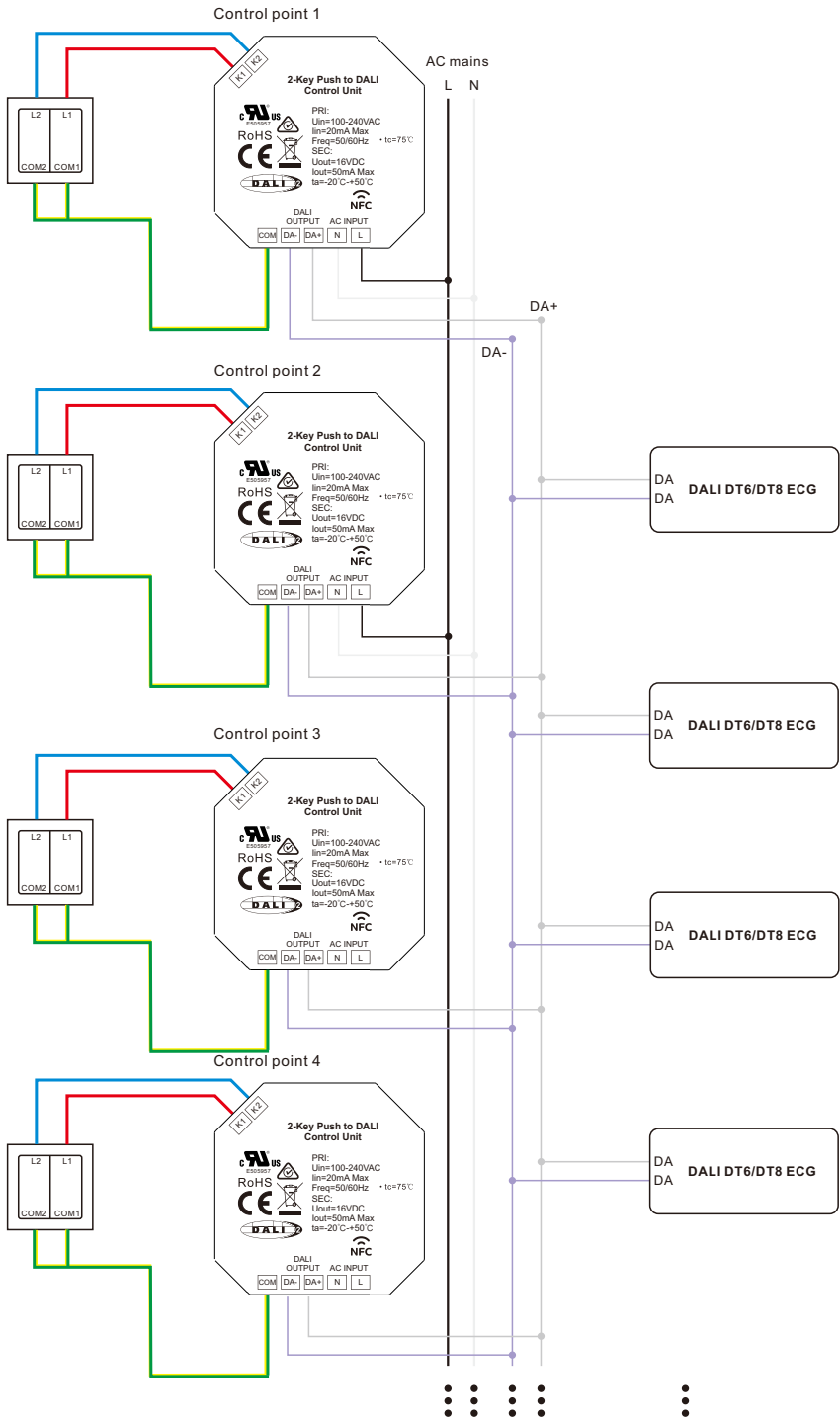
Figure 2: Wiring scheme to control up to 50 DALI ECGs (2 control units powered by AC mains, the other 2 powered by DALI bus)
