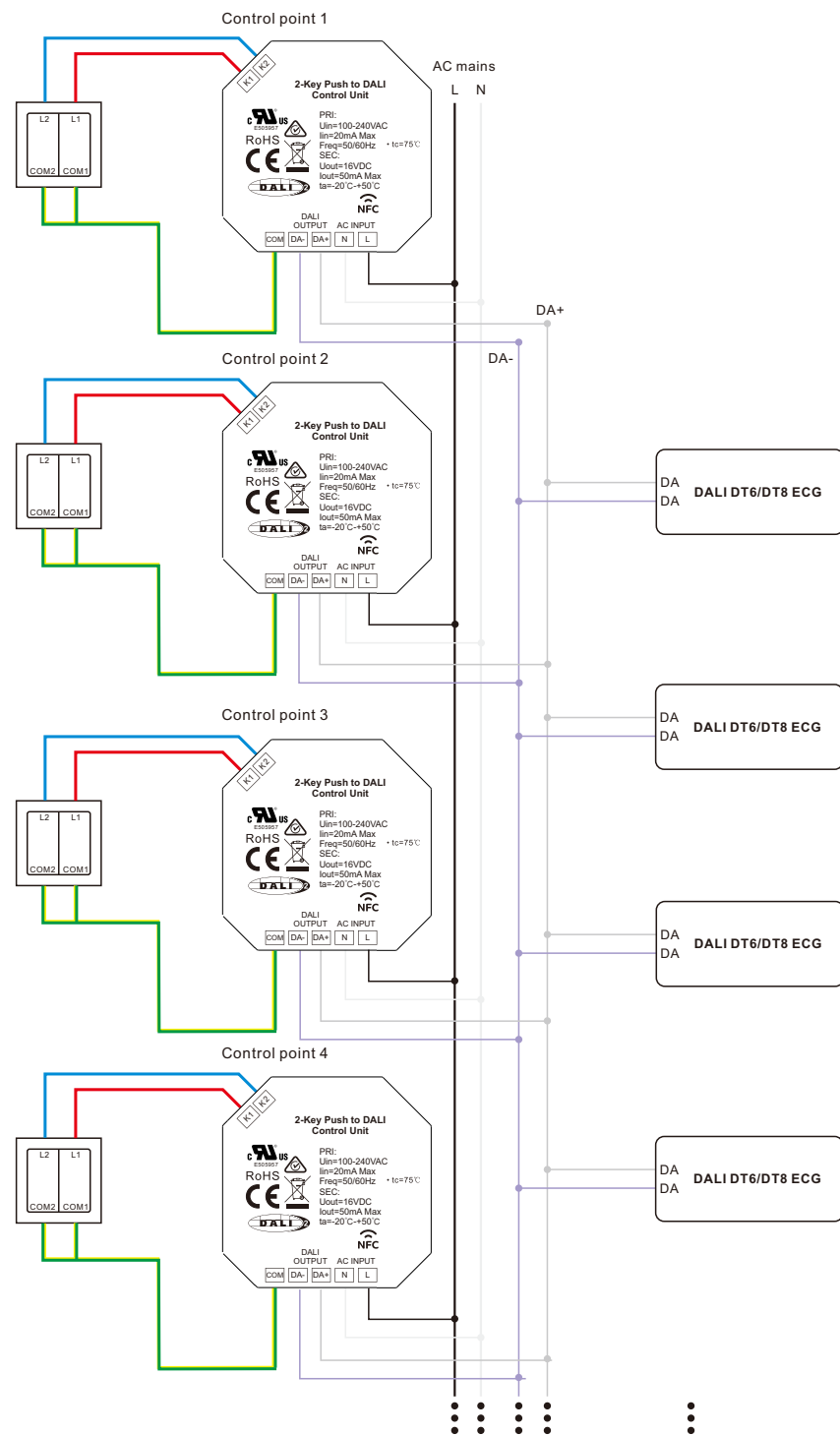
Figure 4: Wiring scheme to control up to 100 DALI ECGs (all 4 control units powered by AC mains)
