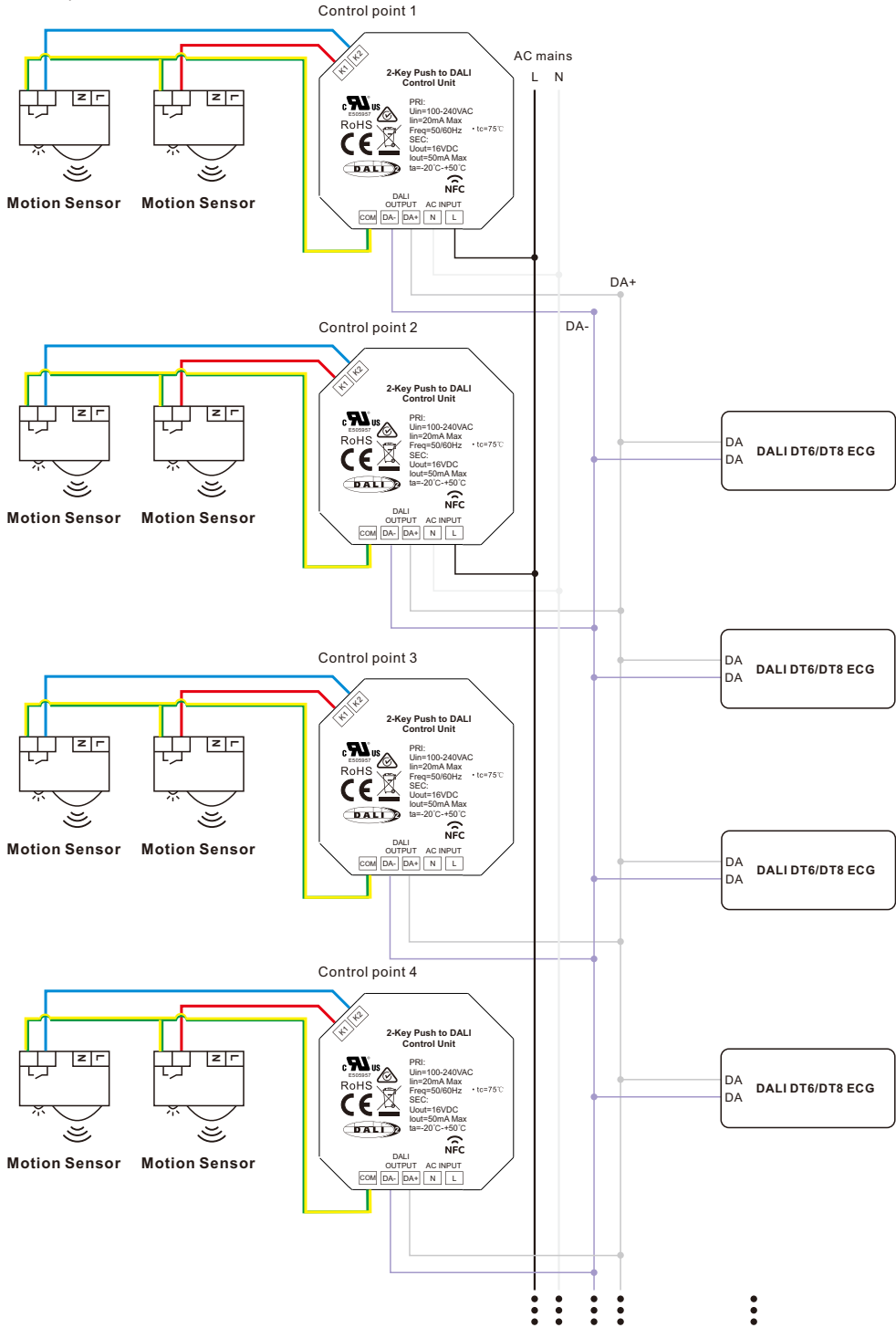
Figure 2: Wiring scheme to control up to 50 DALI ECGs (2 control units powered by AC mains, the other 2 powered by DALI bus)
