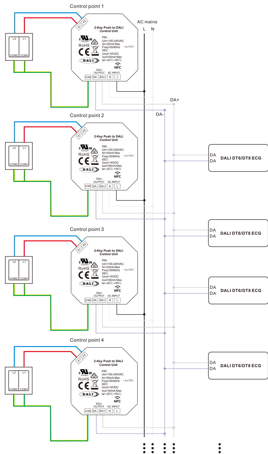
Figure 3: Wiring scheme to control up to 75 DALI ECGs (3 control units powered by AC mains, the other 1 powered by DALI bus)
